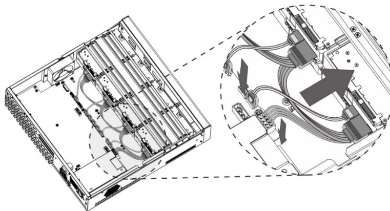
Figure 2-14 Conectar cables
