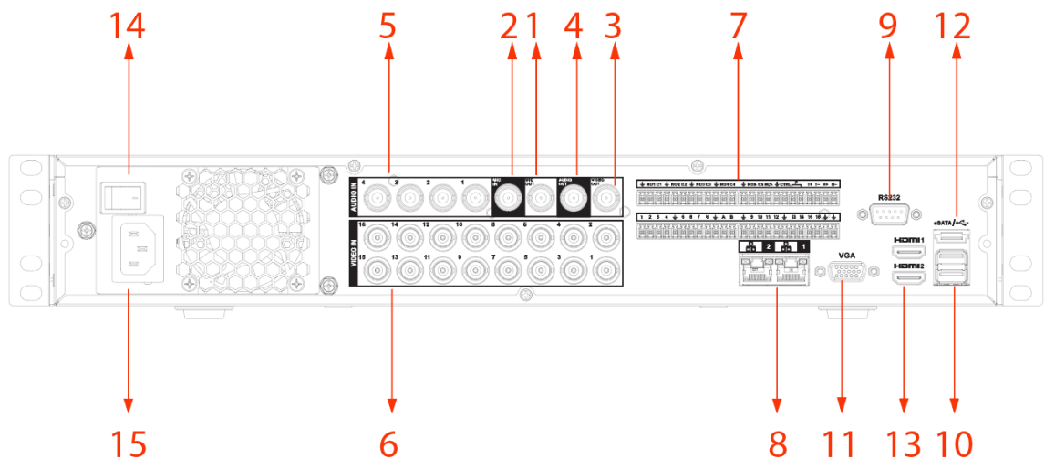
Figure 3-20 Panel trasero (3)
