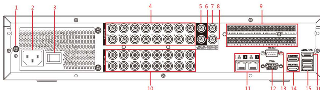
Figure 3-16 Panel trasero
