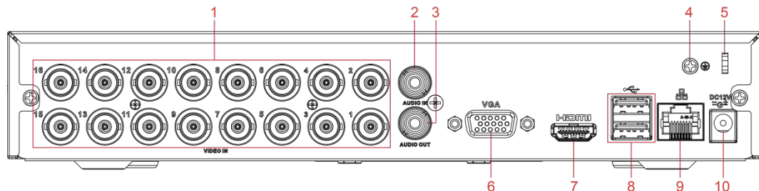
Figure 3-21 Panel trasero
