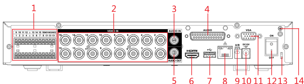
Figure 3-12 Panel trasero
