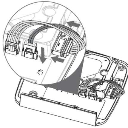
Figure 2-33 Conectar cables
