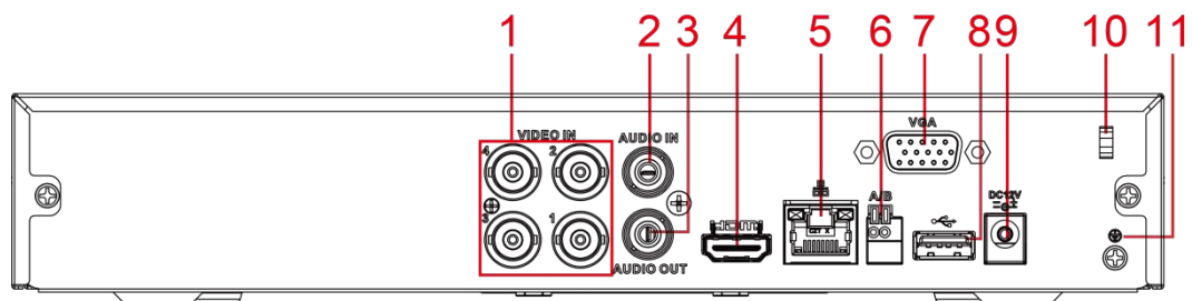
Figure 3-13 Panel trasero
