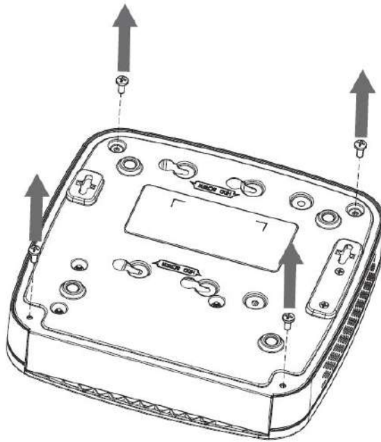
Figure 2-30 Remove screws
