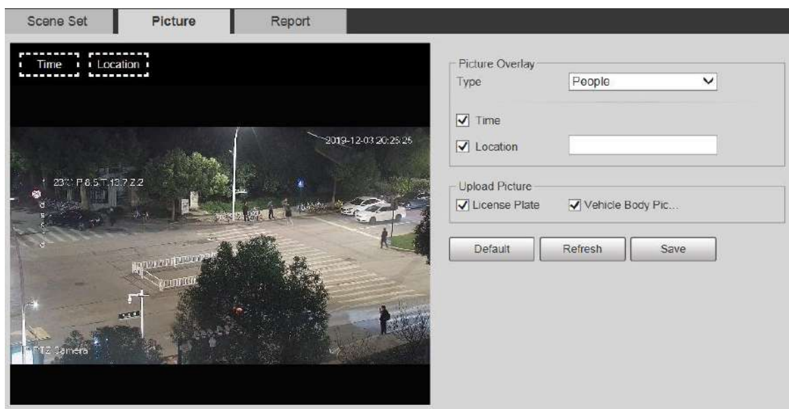
Figure 5-116 Picture overlay–people
