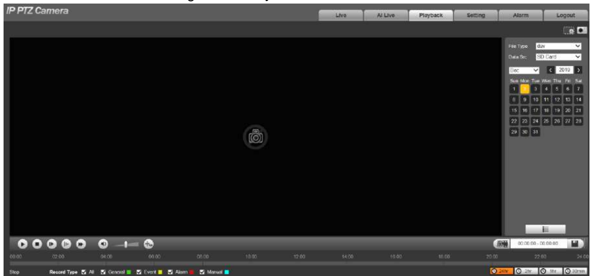
Figure 4-1 Playback interface
