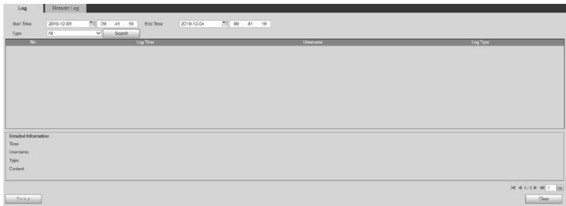
Figure 5-167 Log
