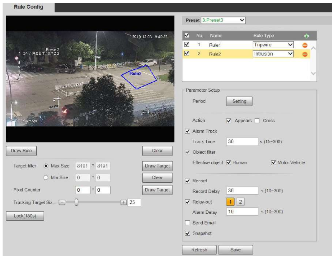
Figure 5-91 Intrusion settings
