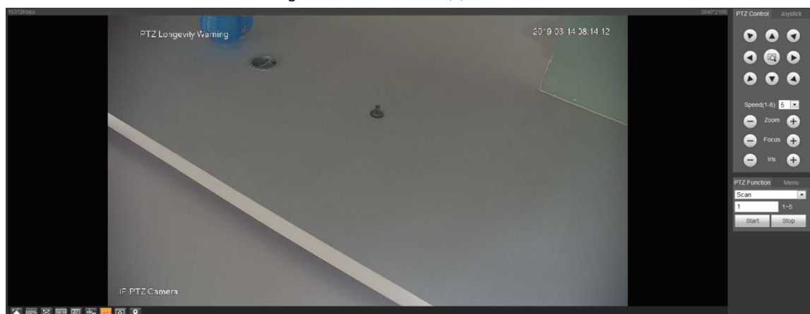
Figura 2-24 Advertencia (2)
