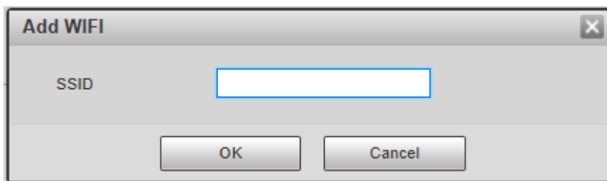
Figura 5-50 Agregar Wi-Fi
