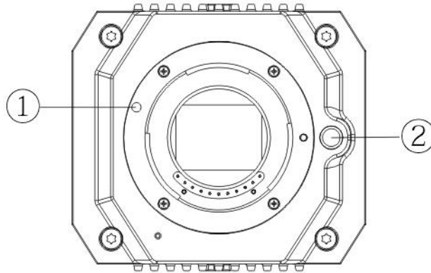
Figure 9-2 Front panel
