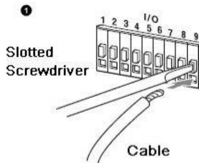
Figure 9-4 Install cable
